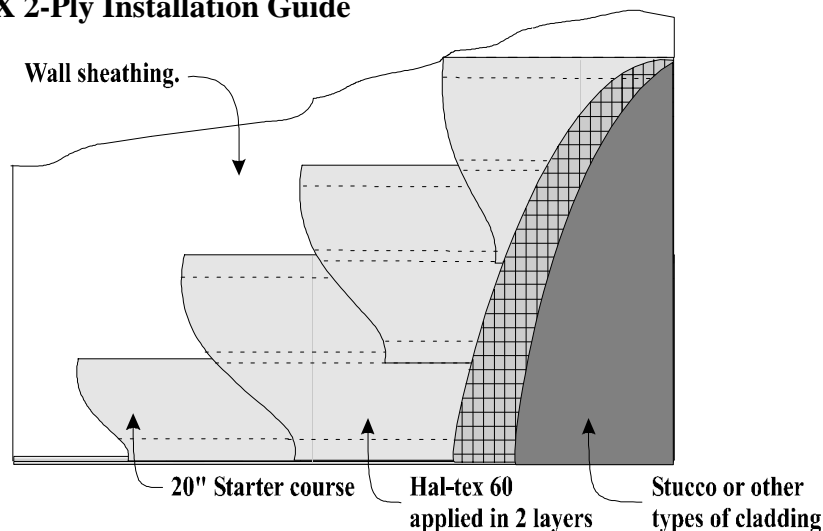
Figure 1: HAL-TEX 2-Ply Installation Guide
